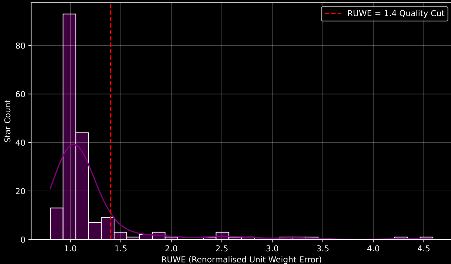
GAPOGEE DR17 Field [K2_C13_173-16_btx] RUWE Distribution (n= 187)
