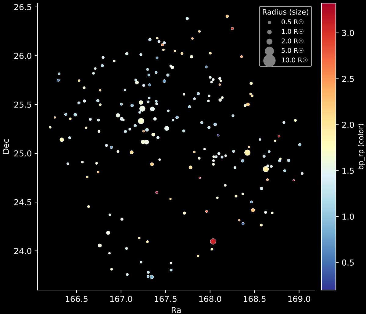
APOGEE DR17 Field: [K2_C13_173-16_btx] Stars: 193
