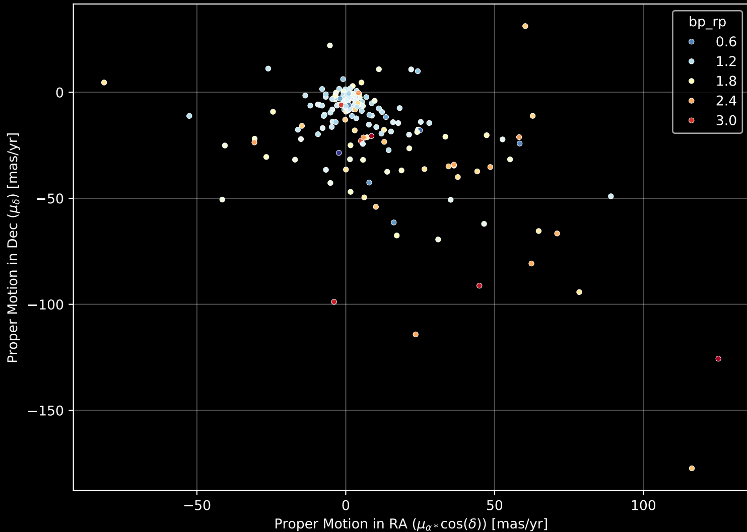
APOGEE DR17 Field: [K2_C13_173-16_btx] Proper Motion Diagram (n= 193)
