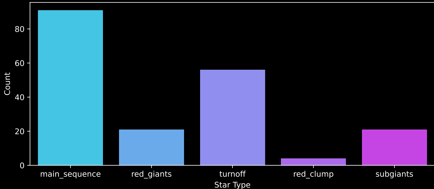
APOGEE DR17 Field: [K2_C13_173-16_btx] Count plot of Star Type
