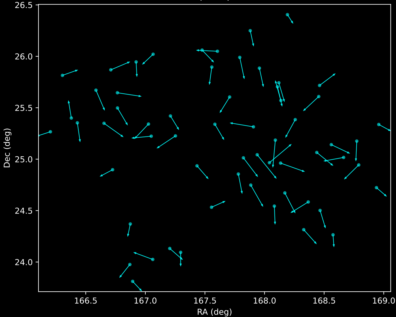
APOGEE DR17 Noise Stream Proper Motion Vectors (n=60)
