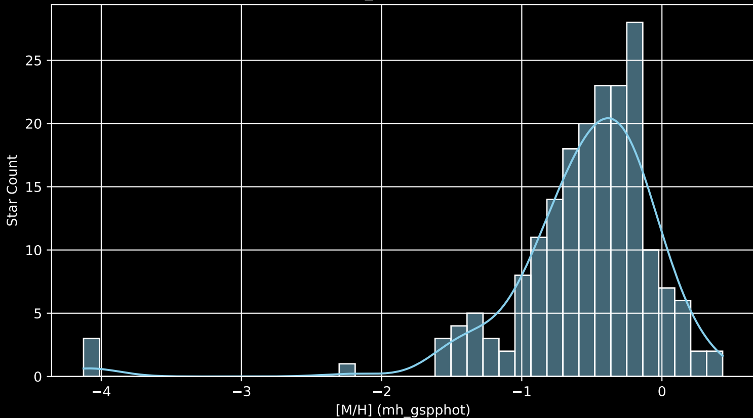
APOGEE DR17 Field: [K2_C13_173-16_btx [M/H] (mh_gspphot) (n= 193)
