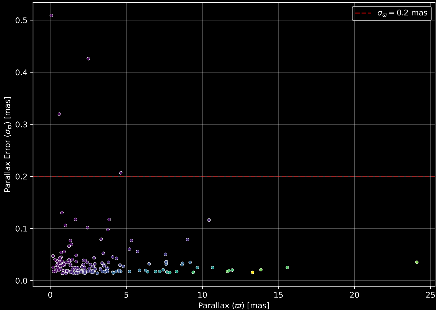
APOGEE DR17 Field: [K2_C13_173-16_btx] Parallax Quality (n= 193)
